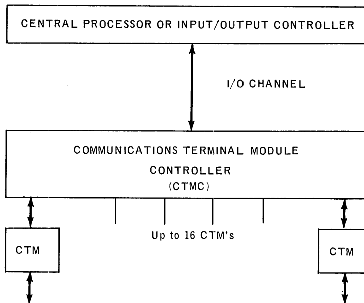
Figure 9-1. CTMC Subsystem
